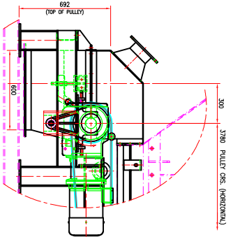
DETAIL - D1 ENLARGED DETAILS OF HEAD END PULLEY
