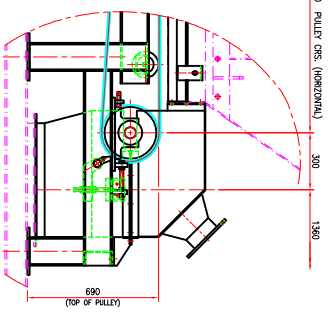
DETAIL - D2 ENLARGED DETAILS OF TAIL END PULLEY
