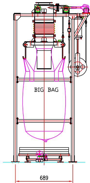
END VIEW
